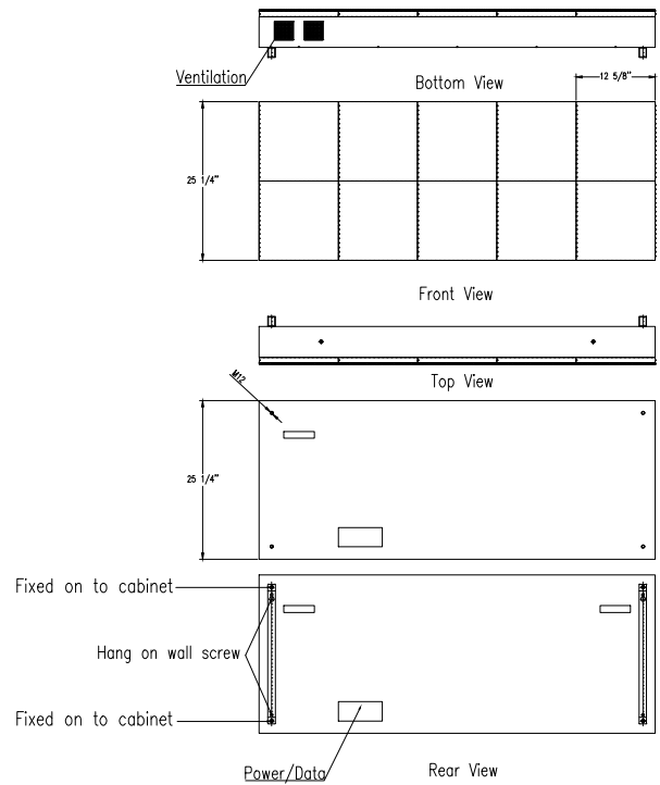
TYPE 1 MOUNTING: HANDY HANG
